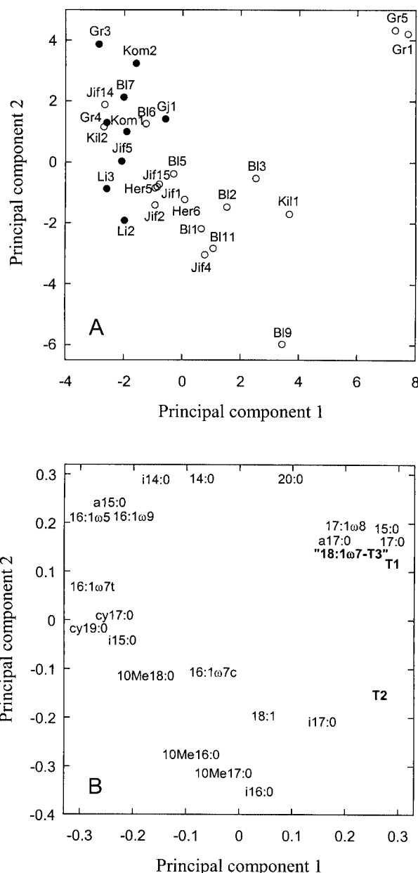
FIG. 1. PCA of the PLFA pattern of self-heated (open symbols) and unheated (solid symbols) peat. BI, Bliksrud; Gr, Grenimosan; Her, Herremyr; Kil, Killingmo; Jif, Jif peat; GJ, Gjødalsmosan; Kom, Komnes; Li, Liermosan. For background data, see Table 1. Samples denoted Jif2, Jif4, Jif14, and Jif15 were subjected only to PLFA analyses and are therefore not included in the table. (A) Score plot of the different peat samples. (B) Loading plot of the individual PLFAs. The PLFAs T1, T2, and 18:1 \omega 7-T3 are in bold.
