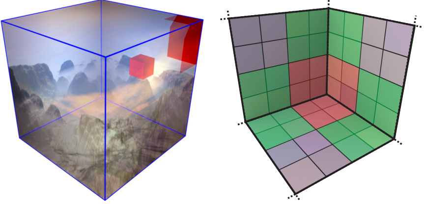
Figure A.3: Left : The cube mapping problem. A texture coordinate interval (the red box) may map to several sides on the cube (the projection of the red box), but current hardware only allows one side at a time to be accessed. Right : Min-Max mipmap generation for interval-based cube mapping. Only a small part of the cubemap is shown here. We use texels from both sides of an edge (the green regions), and texels from three sides in the corners (the red region).
