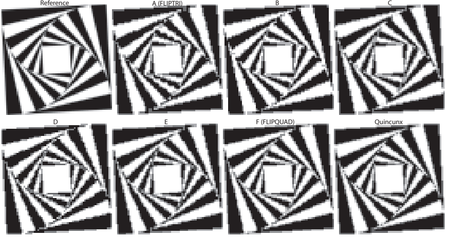
Figure 5: A spiral test image rendered using the sampling schemes, A through F, from Figure 3. The reference image is supersampled with 1024 jittered grid sample points and uses a 4 \times 4 pixel Michell-Netravali reconstruction filter. An image rendered using the Quincunx pattern is also included for comparison.
