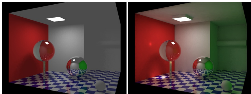
Figure 2: Left: An image rendered with a simple light model, not including any indirect lighting. Right: The same image rendered with a physically based lighting model. Note that a great deal of the light in this scene actually comes from indirect lighting. As a result, the rendered image to the right looks more realistic, and it also makes it easier to perceive the depth and shape of the scene.
