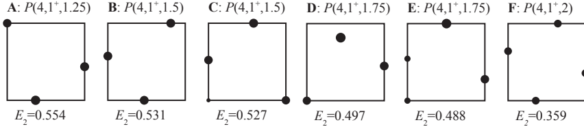
Figure 3: The figure shows the best schemes in terms of the error metric E_2 in each class. The area of each circle is proportional to the weight of the corresponding sample point. For n = 1.5 and n = 1.75 , two patterns were found with similar error measures, but with different number of samples used during reconstruction. Schemes A and F are versions of the FLIPTRI and FLIPQUAD schemes respectively, that have been optimized using the E_2 error metric (see section 5.2)
