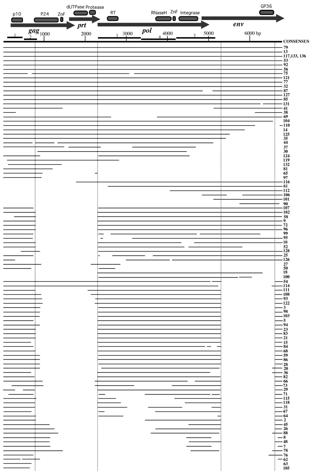
FIG. 1. Structures of 100 HERV-K(HML-5) provirus sequences. An ORF map of the HERV-K(HML-5) consensus sequence generated in this study, including retroviral gag , pri , pol , and env reading frames and protein domains, is shown at the top. Structures of proviral sequences with regard to the consensus sequence are depicted below, with horizontal lines indicating the presence of respective proviral portions. Numbers to the right refer to proviral locus numbers given in Table 1. Proviruses 117, 133, and 136 probably stem from genomic duplication events and are
