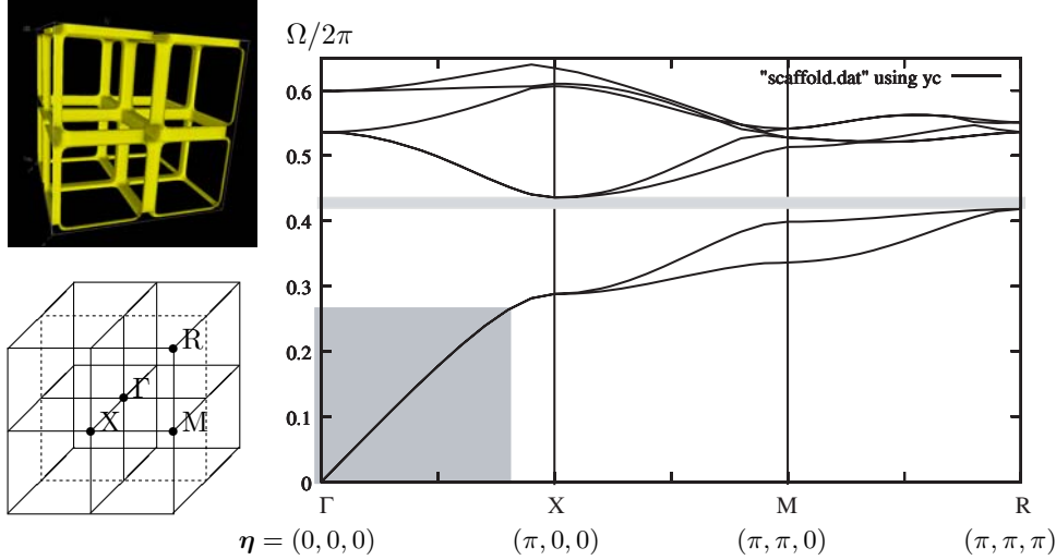
FIG. 6.1. Plot of a typical band structure. The eigenvalues \Omega_n for the geometry in the upper left figure (unit cell U = ]0, 1[^3 ) are depicted as functions of the wave vector \boldsymbol{\eta} in the reciprocal unit cell U' = ]-\pi, \pi[^3 in the lower left figure. The shaded area in the lower left part of the diagram indicates the approximate validity range of classical homogenization [23]. The thin grey strip is a band gap, where there are no eigenvalues regardless of the wave vector. Thus, in this frequency interval there can exist no fixed frequency solutions to Maxwell's equations. In this plot, the optical modes are above the band gap, and the acoustic modes are below. There are only two acoustic modes, since we do not plot the negative frequencies corresponding to propagation in the negative \boldsymbol{\eta} -direction. The calculations are made with the program described in [15], and the scaffold geometry is taken from [9]. The thickness of the bars is 20% of the unit cell, and the permittivity in the bars is 12.96.
