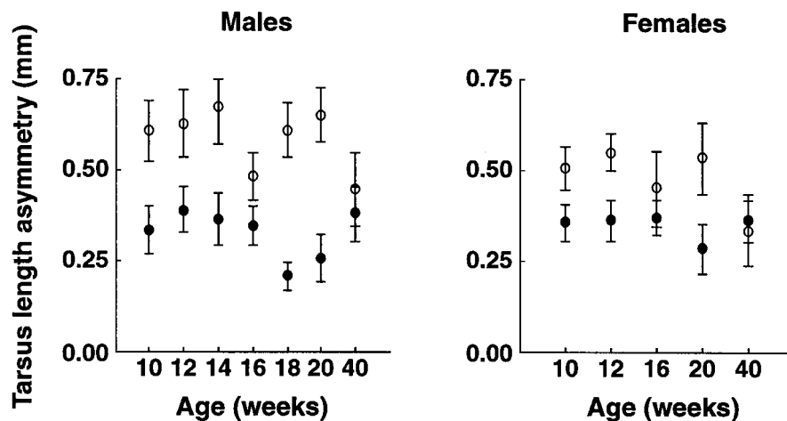
Figure 3. Fluctuating asymmetry ( |L - R| , \pm SE) in tarsus length of male and female pheasants in relation to experimental treatment during the first 3 wk of life. Chicks either received high- (closed circles) or low- (open circles) protein food. Only males were measured at weeks 14 and 18.
