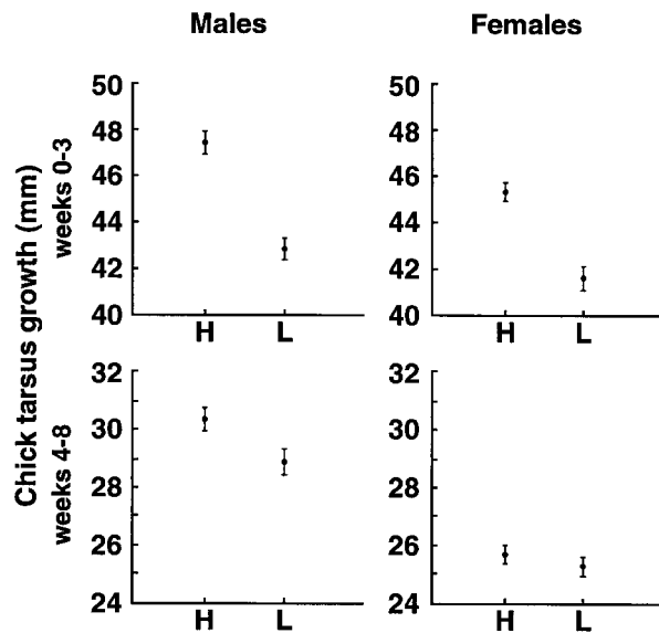
Figure 1. Growth of chick tarsus length ( \pm SE) during the early experimental period (first 3 wk, upper panels) and during the late experimental period (subsequent 5 wk, lower panels) for males and females. The chicks received either high-protein food (H) or low-protein food (L). Means in the lower panels are adjusted for unequal sample size of the early treatment in each group. Error bars for the lower panels calculated using residuals from one-way ANOVAs including early treatment as factor.
