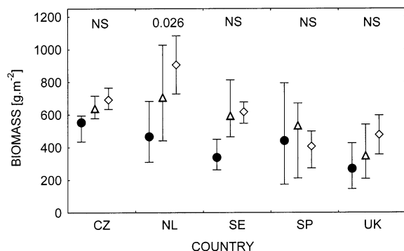
Fig. 3. Minimum, average and maximum biomass in NC (●), LD (△) and HD (◇) treatments. Minimum and maximum (whiskers) are extreme values among the five blocks, value for each block being average based on twelve 0.0625-m 2 plots. The values shown are the significance values for the comparison of averages derived from a separate ANOVA for each country (with block as a random factor), comparing the LD and HD treatments only, NS means P > 0.1 .
