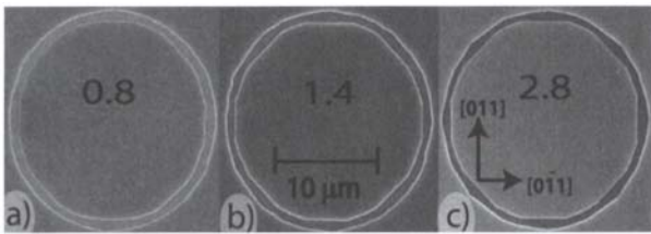
Figure 3. V/III ratio effect on the selective epitaxy over 1 \mu m wide W rings: a) V/III=0.8 b) V/III=1.4 c) V/III=2.8
