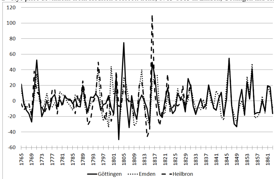
Figure 2 - Rye price deviations from Hodrick-Prescott trend, 1765-1863 in Emden, Göttingen and Heilbron
