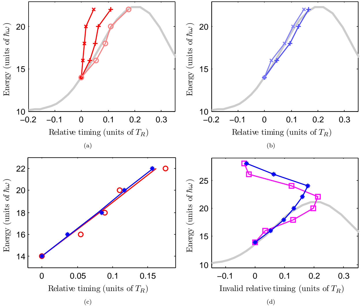
FIG. 5: (Color online) (a) RABITT measurements with one (+) and two ( \times ) aluminum filters are used to determine the relative timing of the unfiltered attosecond pulses ( \circ ). All temporal measurements are presented as relative timings with reference to harmonic 14. (b) In-situ measurements with one (+) and two ( \times ) aluminum filters. The data is uncorrected, \gamma = 1 . The simple classical model ( I_R = 1 \times 10^{14} W/cm ^2 ) [5(a)-5(b) gray curve] is plotted for reference. (c) Unfiltered RABITT measurement (red \circ ) compared to the average in-situ measurement (blue * ). (d) A slight increase of the blue intensity (blue * ) has a small effect on the measurement in the harmonic plateau (harmonic 14 – 24). Increasing the blue intensity further (pink \square ) results in an invalid measurement. The simple classical model ( I_R = 0.9 \times 10^{14} W/cm ^2 ) [gray line] is plotted for reference. Beyond the cut-off (harmonic 24 – 28), a similar shift occurs as for the long branch in Fig. 3(b).
