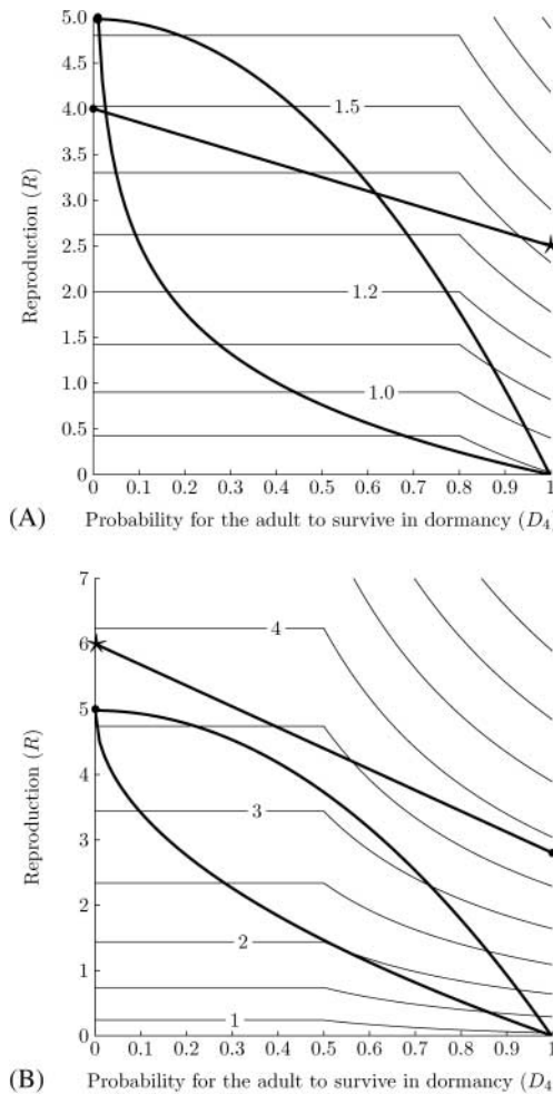
Fig. 3. Contour lines of the fitness landscape in a positively autocorrelated environment (equation 6), depicted as a function of adult dormant survival ( D_4 ) and per capita reproduction ( R ). The bold lines illustrate three possible trade-off curves: a linear, a convex and a concave trade-off. Solid circles denote global fitness maxima and stars indicate local fitness maxima. Parameter values according to Table 1, except in (B) D_2 = 0.5 .
