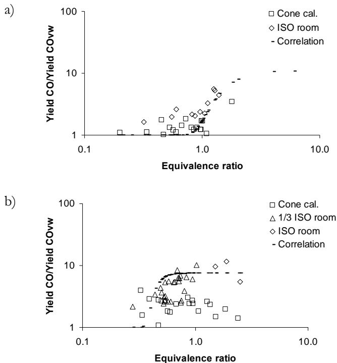
Figure 18. a) Ratio of the yield of CO to the CO yield for well-ventilated conditions during experiments with PP. The dashed line shows the Tewarson correlation. b) Ratio of the yield of CO to the CO yield for well-ventilated conditions during experiments with CB. The dashed line shows the Tewarson correlation.
