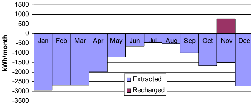
Figure 7.17 Heat extracted from the borehole in a simulation of system 1 (no solar heat) when heat is recharged just during November with an auxiliary heater (1.7kW) for a system with 100 m borehole and the power of heat pump 7kW_{th} . Reference case: Stockholm climate, about 29 400 kWh/year heat and DHW demand, result from the 3 rd year of operation.
