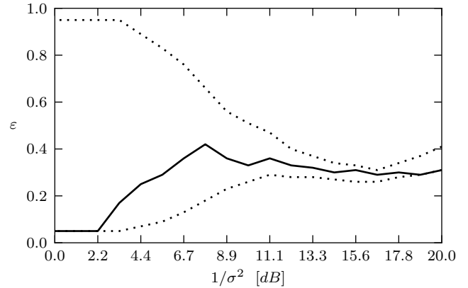
Fig. 2. Optimal Thresholds T_{\text{tr}} (i.e., \varepsilon ) for the BEAST using different noise standard deviations \sigma
