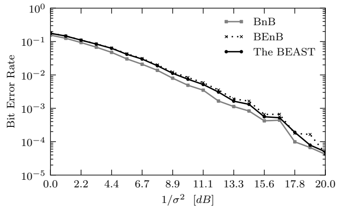
Fig. 3. Obtained bit error rate for a given noise standard deviation \sigma for all three algorithm approaches using packet length of T = 50
