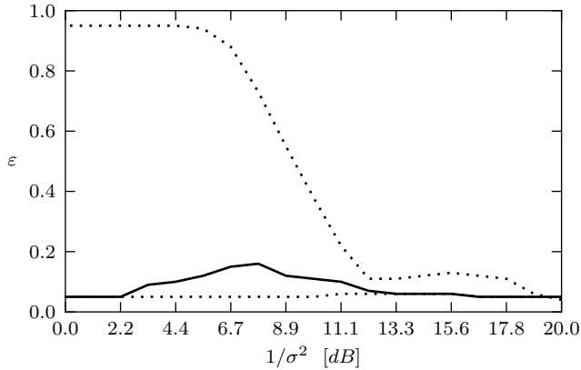
Fig. 1. Optimal Thresholds T_{\text{tr}} (i.e., \varepsilon ) for BEnB using different noise standard deviations \sigma
