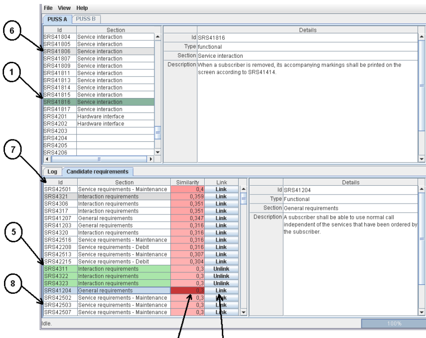
Figure 5.3: The user interface of ReqSimileA used in the experiment.
