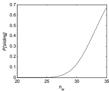
Figure 6-6 – Example of fragility curve for sliding of a concrete gravity dam. h_{rwl} = 20m in this case.
