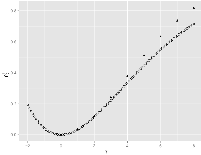
Figure 2 The joint correlation coefficient \rho_J^2 calculated for \gamma ranging from -2 to 8 for bicomponent models with (\alpha; \beta) parameter values (2.1, 2.4; 2.2, 2.3) ( \circ ) and tricomponent models with (\alpha; \beta) parameter values (2.1, 2.4, 2.3; 2.2, 2.3, 2.1) ( \blacktriangle ).
