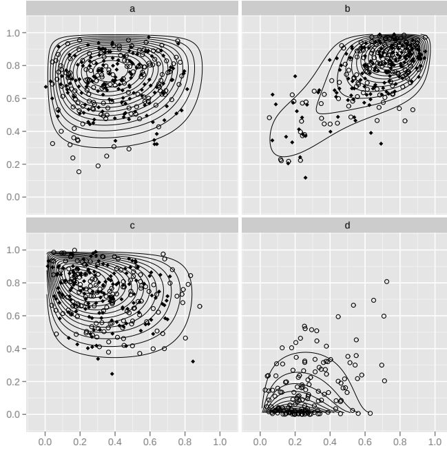
Figure 2 150 random variates generated from four different bicompositional bicompositional Dirichlet distributions with (\alpha; \beta; \gamma) parameters (2.1, 3.1; 5.5, 2.3; 0.3) (a), (2.1, 3.1; 5.5, 2.3; 7.7) (b), (2.1, 3.1; 5.5, 2.3; -1.2) (c), and (2.1, 3.1; 0.7, 2.3; 3.2) (d), using the product of two Dirichlet densities ( \circ ) and a uniform density ( \blacklozenge ) as dominating density. Since the distribution in (d) does not have an upper bound, a uniform density may not be utilized. As a reference, the contour curves of the true densities are also drawn.
