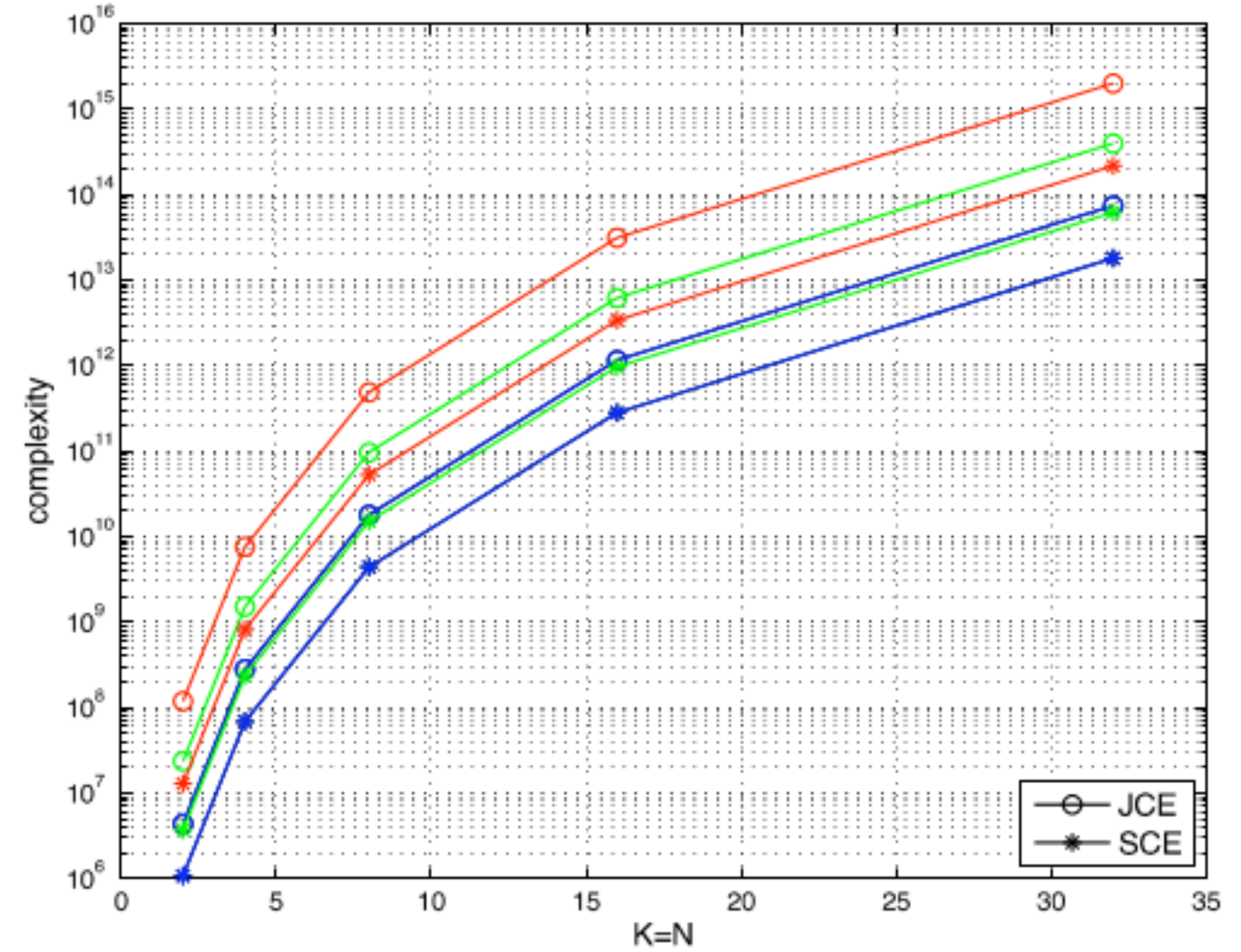
Fig. 3. Computational complexity of JCE and SCE, for M = 64 and \nu_{\max}^{(D)} = 0.05 , in the following cases: (i) S = 64 , \eta_{\max}^{(d)} = 0.05 in blue; (ii) S = 80 , \eta_{\max}^{(d)} = 0.07 in green; (iii) S = 96 , \eta_{\max}^{(d)} = 0.1 in red.
