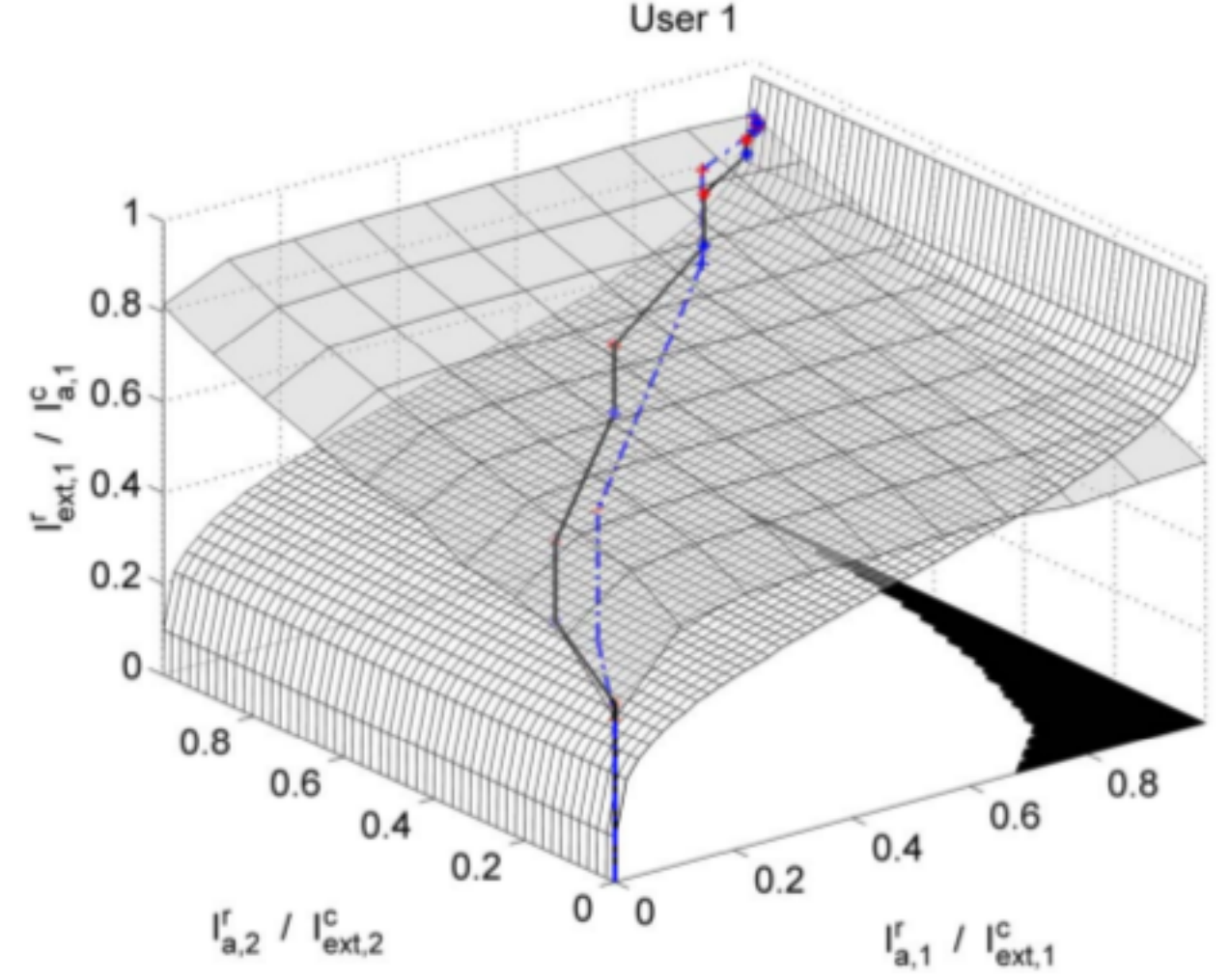
Fig. 6. EXIT chart for user 1. The solid line show an actual decoding trajectory and the dashed line the EXIT chart prediction.
