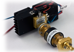
Fig. 4. Photo of HBV X5 transmitter module.
