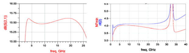
Figure 4. Simulated LNA gain, NF min and NF
