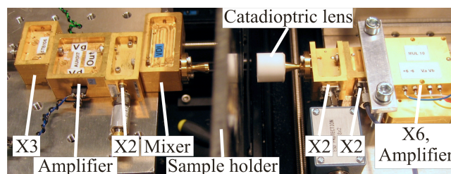
Fig. 2 The constructed 340 GHz heterodyne imaging setup in transmission-mode.
