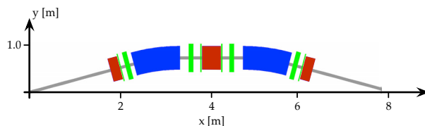
Figure 5: Schematic of one of the twelve DBAs of the MAX IV 1.5 GeV storage ring. Magnets indicated are gradient dipoles (blue), combined quadrupole/sextupole magnets (red), and discrete sextupoles (green).
