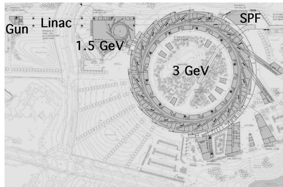
Figure 1: Overview of the MAX IV facility. The gun bunker is at the top left followed by the underground linac tunnel. The 1.5 GeV and 3 GeV storage ring buildings are indicated. The SPF is indicated at the top right.
