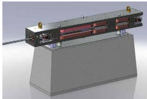
Figure 4: Illustration of the solid iron block out of which the magnets for one complete cell of the MAX IV 3 GeV storage ring have been machined. The example here shows the matching cell upstream of the long straight section. Note the massive concrete support with mounting plate.
