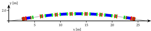
Figure 2: Schematic of one of the 20 achromats of the MAX IV 3 GeV storage ring. Magnets indicated are gradient dipoles (blue), focusing quadrupoles (red), sextupoles (green), and octupoles (brown). The basic structure of five unit cells flanked on either side by a matching cell can be recognized.
