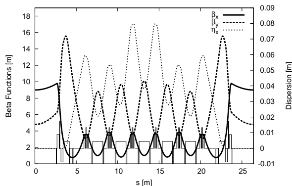
Figure 3: Beta functions \beta_x, \beta_y and dispersion \eta_x for one achromat of the MAX IV 3 GeV storage ring. The position of the dipoles, quadrupoles, sextupoles, and octupoles are indicated at the bottom.
