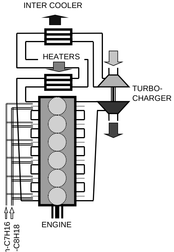
Figure 1 Engine system.
