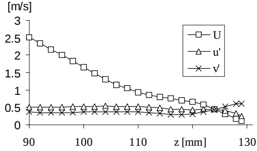
Figure 9. Centerline velocities at \lambda = 1.69 , U_{\text{exit}} = 4.11 m/s, Z = 131 mm and d = 10 mm.
