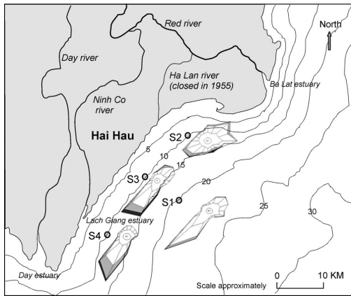
Figure 5. Current prisms based on short-term series of measured data in 2005 and 2006 at four anchored stations.
