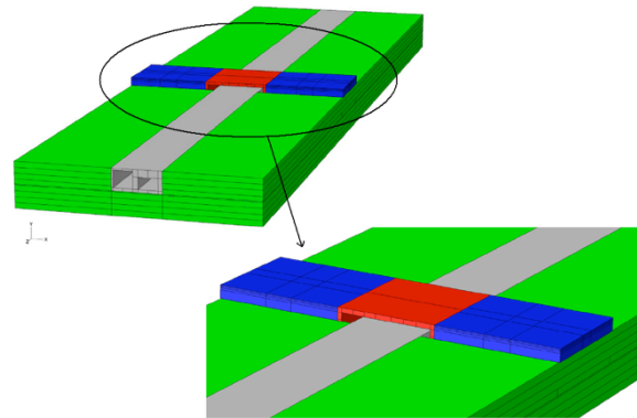
Figure 2 : Finite Element Model
