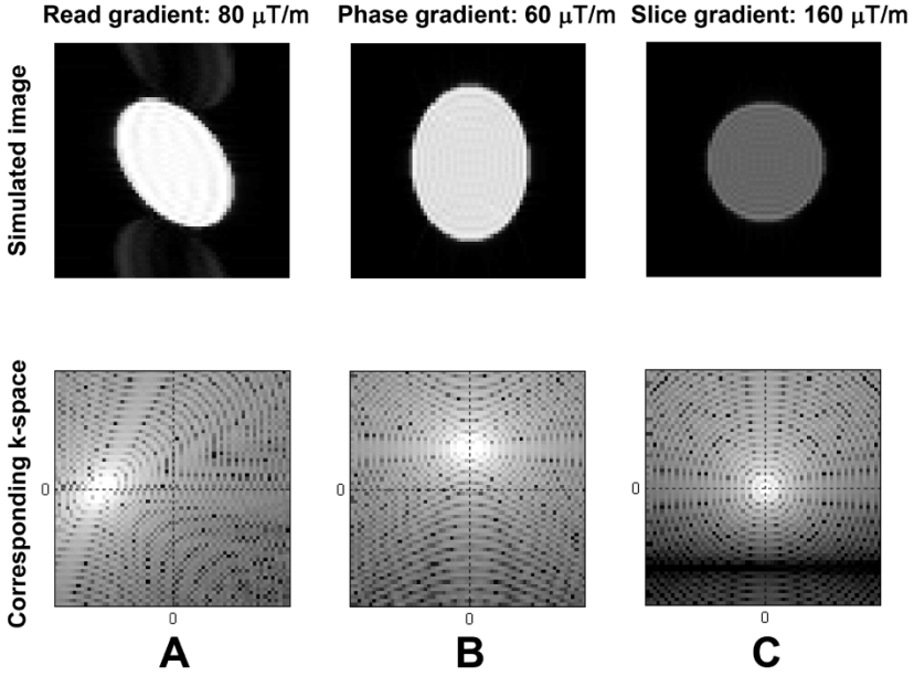
Figure 3.2. Simulated images of a cylindrical object (top row) and the corresponding k -space (bottom row) showing the effects of uniform linear gradients in: (A) the readout direction (80 \mu\text{T/m} ), (B) the phase-encoding direction (60 \mu\text{T/m} ) and (C) the slice selection direction (160 \mu\text{T/m} ).
