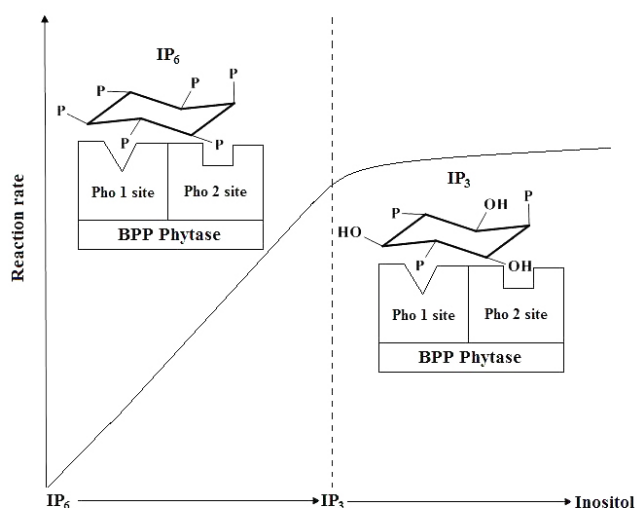
Figure 3.4 Scheme of phytate hydrolysis by TS-Phy (redrawn according to Shin et al. [232]). The reaction is fast when two adjacent phosphate groups of the substrate simultaneously occupy both the cleavage (Pho1) and the affinity (Pho2) sites. The reaction is very slow when only one phosphate group occupies the cleavage site (Pho1), and the affinity site (Pho2) is empty. P stands for H_2PO_4^- .
