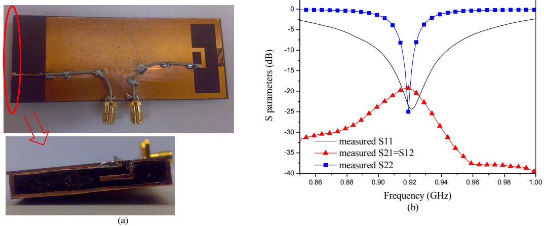
Figure 4. The (a) fabricated prototype and (b) measured S parameters of the proposed antenna system.
