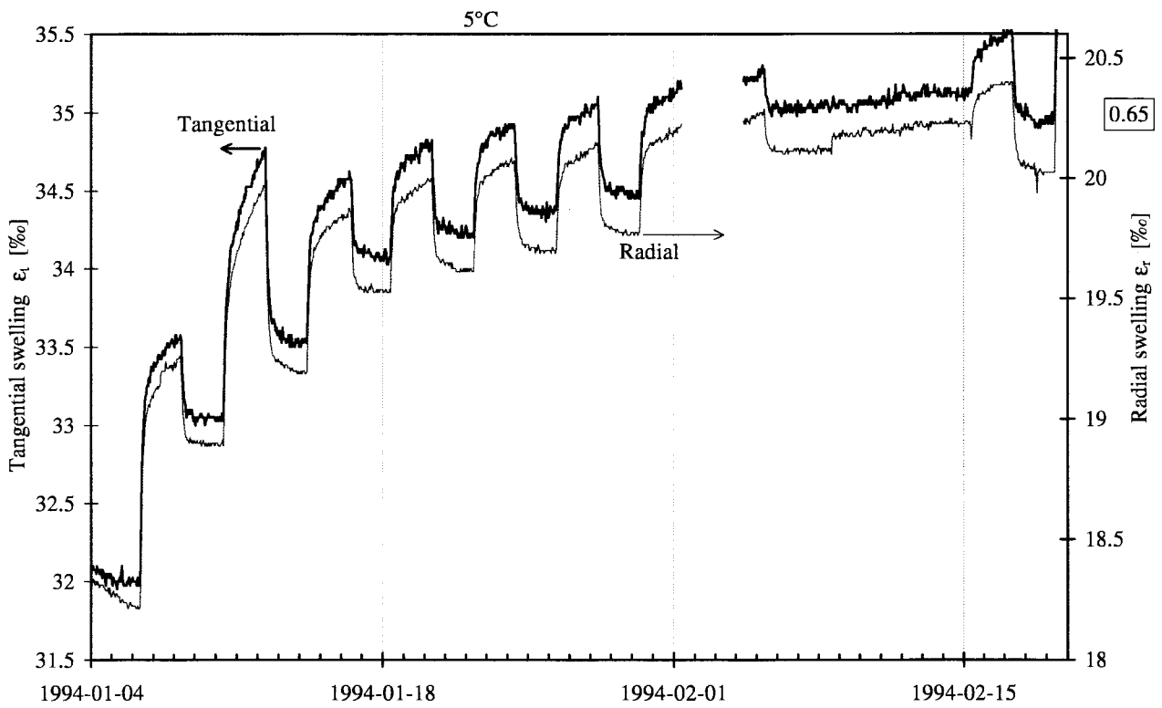
Figure 6.51 Tangential and radial swelling responses, 88% ↔ 90% cyclic RH-steps.
