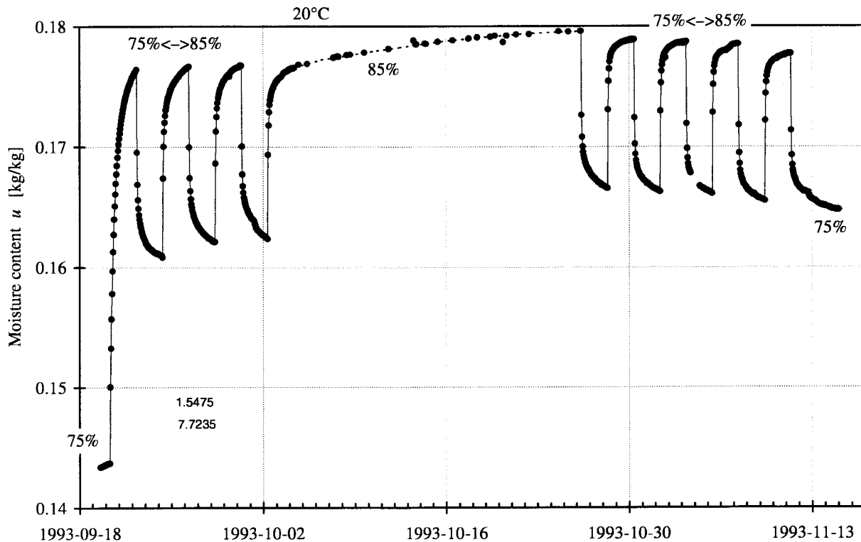
Figure 6.41 Sorption response, Sample 3, 75% \leftrightarrow 85% cyclic RH-steps.
