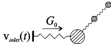
Figure 10.3 Network for the thin samples of the experiments. Outer node in contact with the climate chamber and two internal levels.
