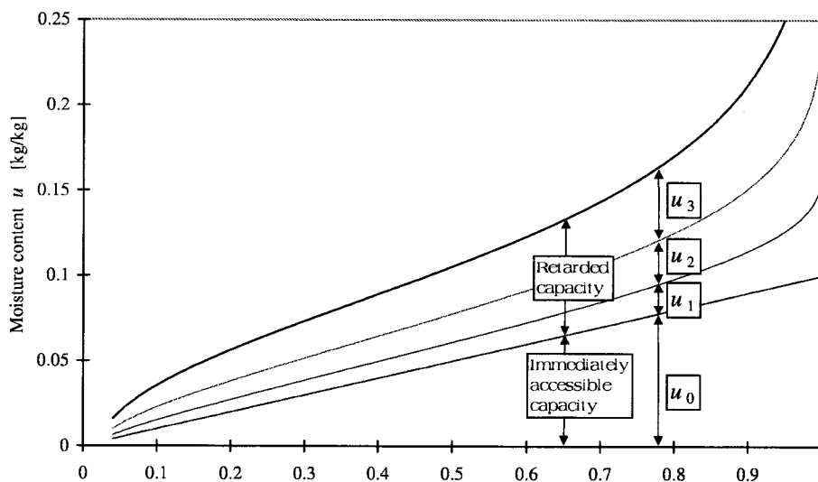
Figure 10.11 Distribution of moisture capacity in model with three internal levels.
