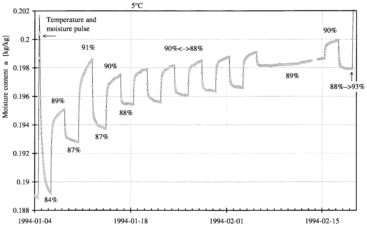
Figure 6.50 Sorption response, Sample 4, 88% ↔ 90% cyclic RH-steps.
