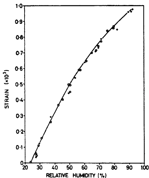
Figure 1.12 Zero-load axial equilibrium dimensional changes plotted against relative humidity. (+) absorption, (°) desorption. From Hunt (1990).
