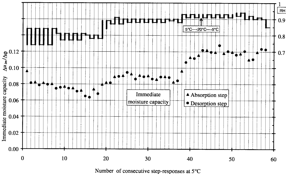
Figure 9.4 Survey of immediate moisture capacity calculated by exponential fitting, Eq. (9.1), for all measurements at 5^\circ\text{C} .
