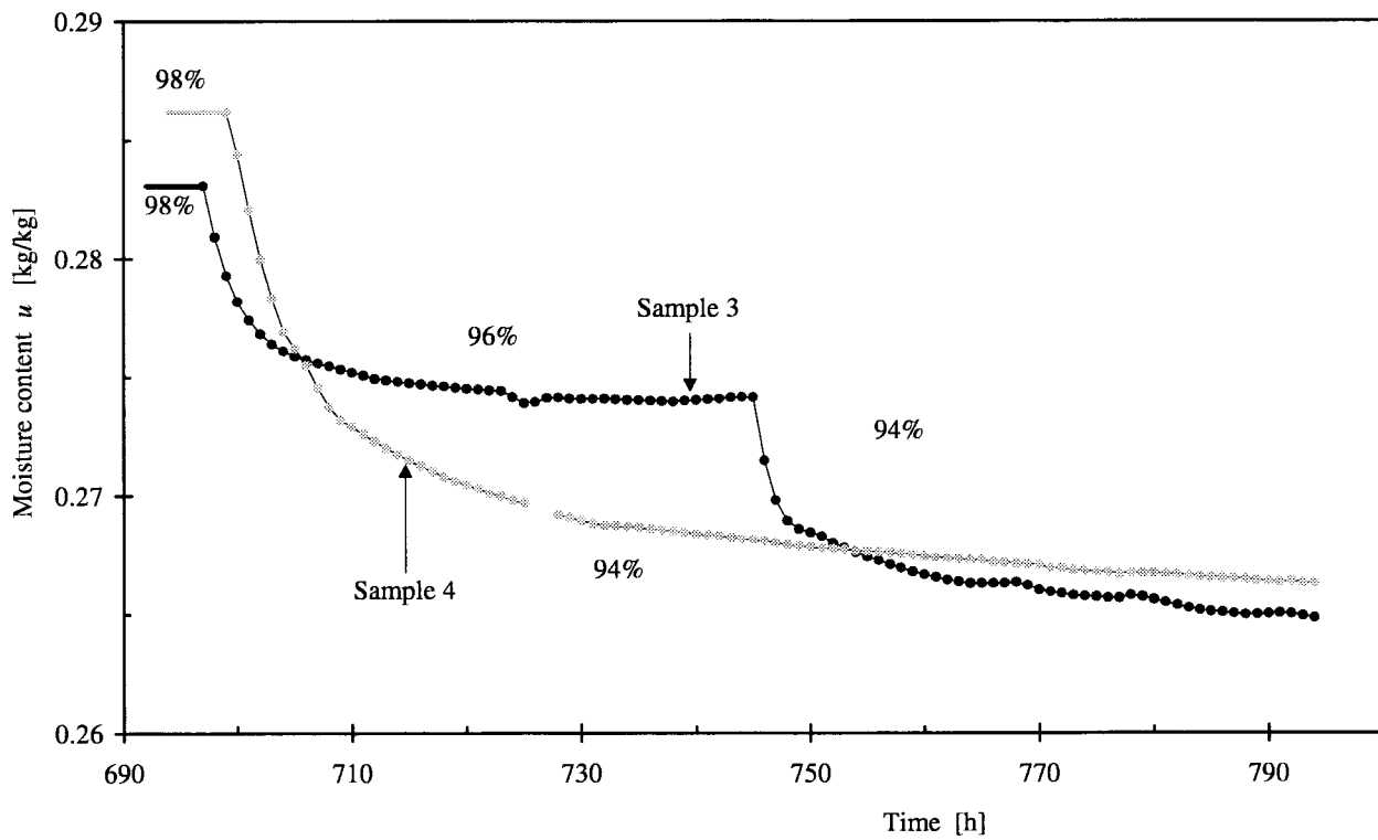
Figure 6.19 Sorption response, Sample 3 and Sample 4, 98% \rightarrow 94% RH-interval.
