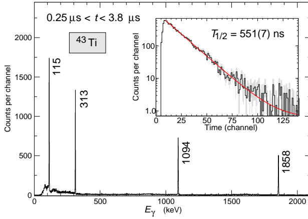
Figure 3. Gamma-ray spectrum taken between 0.25 \mu\text{s} and 3.8 \mu\text{s} after the implantation of ^{43}\text{Ti} ions. The peaks are labelled with their energy in keV. The inset shows the combined decay curve of the 115, 1094, and 1858 keV transitions in ^{43}\text{Ti} . The experimental data are histogrammed in bins of 50 \text{ ns} per channel including an arbitrary offset. The grey area marks the experimental uncertainties. The solid line (red online) corresponds to the result of a least-squares fitting procedure to the exponential decay, including a constant background term.
