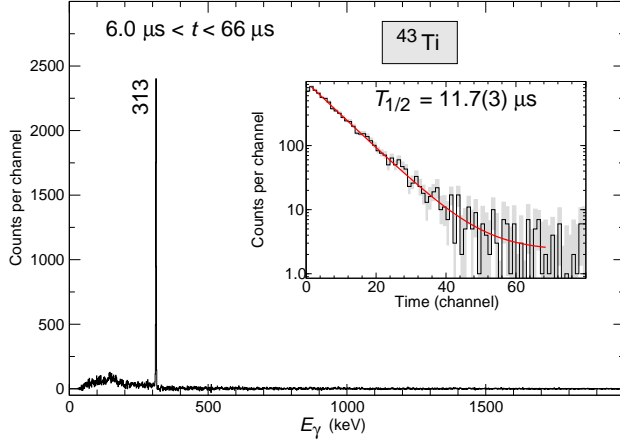
Figure 2. Gamma-ray spectrum taken between 6.0 \mu\text{s} and 66 \mu\text{s} after the implantation of ^{43}\text{Ti} ions. The peak is labelled with its energy in keV. The inset shows the decay curve of the 313 keV transition in ^{43}\text{Ti} . The experimental data are histogrammed in bins of 2 \mu\text{s} per channel, and the grey area marks the experimental uncertainties. The solid line (red online) corresponds to the result of a least-squares fitting procedure to the exponential decay, including a constant background term.
