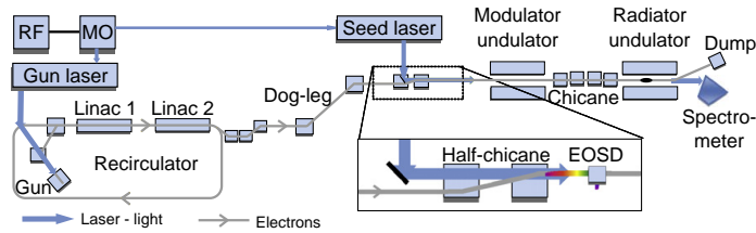
Fig. 1. The test-FEL setup. The electron bunch created by the laser pulse on a photocathode gun passes an energy filter (two dipoles) and a recirculator where it passes through the two linacs twice. The chicane right after the recirculator compresses it. After the dog-leg/transport the electrons are displaced in the half-chicane to insert laser pulses from the seed-laser. Its energy is modulated inside the modulator undulator, turned into density modulation in the chicane and finally radiated on a higher harmonic inside the radiator undulator. The electrons are dumped and the UV radiation continues to the spectrometer. The position of the chamber and the crystal (EOSD) is shown in the enlarged section. The insertion mirror shown in enlarged part before the half-chicane is used as an entrance for all optical pulses.
