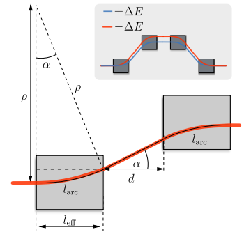
Figure 2.15. One half of a chicane consisting of four dipole magnets. Parameters used in the calculation are shown. The inset figure shows the complete chicane and the fact that the longer path is taken by electrons with an energy lower than the average.
