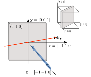
Figure 5.5. The crystal is cut in the (110) plane. In that plane, the field \mathbf{E}_T from electrons makes an angle \alpha relative to the vector \mathbf{x} . The terahertz field and the laser field propagate in the same direction along \mathbf{z} into the crystal.
