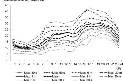
Fig. 4. The average household electric power for the measurement period presented for each clock hour of the day and the maximum and minimum at different intervals ranging from 30 s to 1 h. For example, the values at 8 are based on all data between 07 and 08 in the morning all the measured days. With 1 h resolution, it means one data per day, 5 in total, while it is much more data with 30 s resolution.
