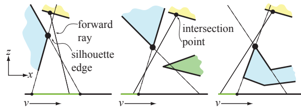
Fig. 6 A multi-view silhouette is clipped in the v -dimension. We use the planes incident to the silhouette edge to limit the extents of the multi-view silhouette edge along the v -axis. The multi-view silhouette edges are clipped to the green intervals on the v -axis. In all three cases, we can only keep the part of the camera line where the edge is a silhouette, and where the intersection point is visible.
