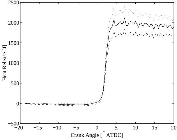
Figure 4.5 Heat release profile for one cycle using \bar{c}_v/\bar{R} = 3.5 (dashed line), and \bar{c}_v/\bar{R} = 4.0 (solid line), and \bar{c}_v/\bar{R} = 4.5 (dotted line).
