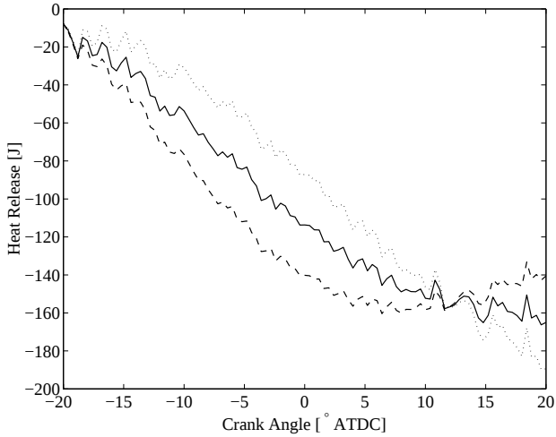
Figure 4.6 Heat release profile for a motored cycle using \bar{c}_v/\bar{R} = 2.5 (dashed line), and \bar{c}_v/\bar{R} = 3.0 (solid line), and \bar{c}_v/\bar{R} = 3.5 (dotted line).
