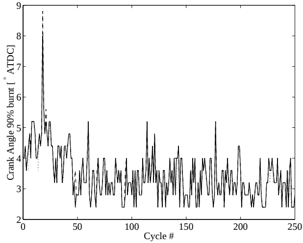
Figure 4.10 Crank angle of 90% burnt for 250 consecutive cycles using \bar{c}_v/R = 3.5 (dashed line), and \bar{c}_v/R = 4.0 (solid line), and \bar{c}_v/R = 4.5 (dotted line).
