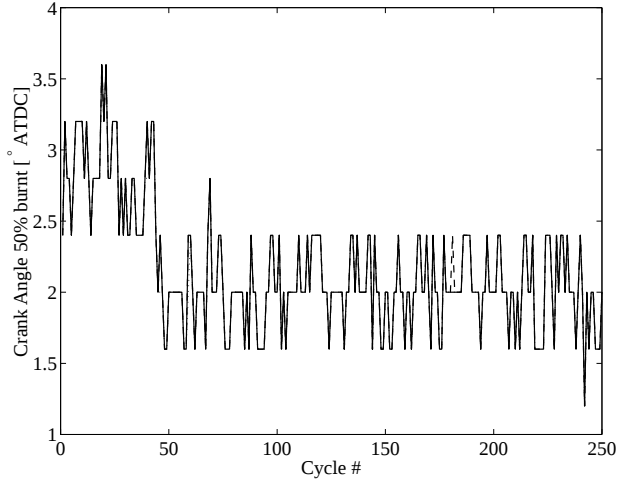
Figure 4.9 Crank angle of 50% burnt for 250 consecutive cycles using \bar{c}_v/R = 3.5 (dashed line), and \bar{c}_v/R = 4.0 (solid line), and \bar{c}_v/R = 4.5 (dotted line).
