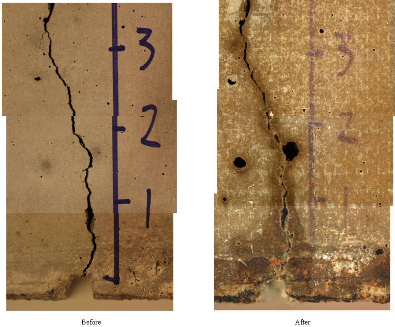
Figure A1.14: Permanently in brackish water. Crack width 0.4 mm. Cover 55 mm. Specimen S155-4-1-2Ö
