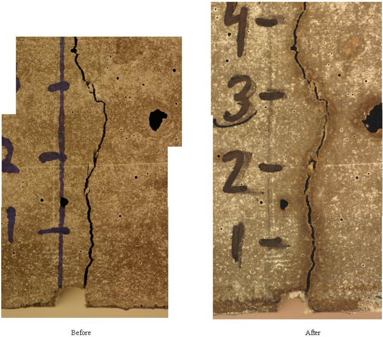
Figure A1.15: Permanently in pure water. Crack width 0.4 mm. Cover 75 mm. Specimen S175-4-1-2R
