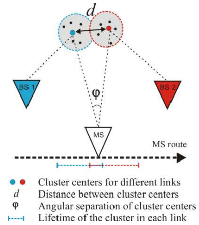
Fig. 4. Extraction of common cluster from measurement data. (a) A flow chart of the procedure for the extraction of common clusters from measurement data. (b) The distance between the scattering points of different links and the angular separation of the scattering points seen from the MS determine if the cluster is considered as common.
