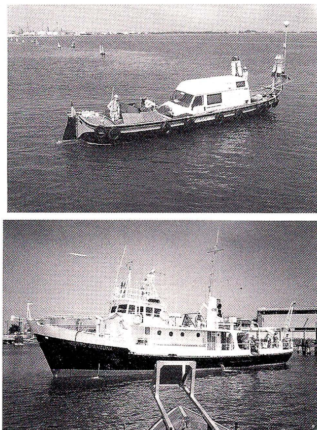
Fig. 3 - a) The lagoon boat hosting the FLIDAR in the Venice lagoon. b) The O/S D'Ancona , taken from the lagoon boat. In the foreground the folding mirror of the FLIDAR, deflecting the laser beam into the water.
