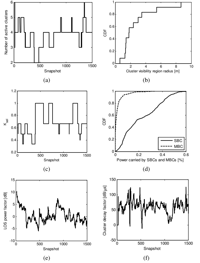
Fig. 3. (a) Total number of active clusters as a function of the MS location. (b) CDF of the visibility region radius. (c) Ratio of single and multiple bounce clusters. (d) Power carried by SBCs and MBCs. (e) LOS power factor. (f) Cluster decay factor. All parameters have been extracted from the reference measurement.
