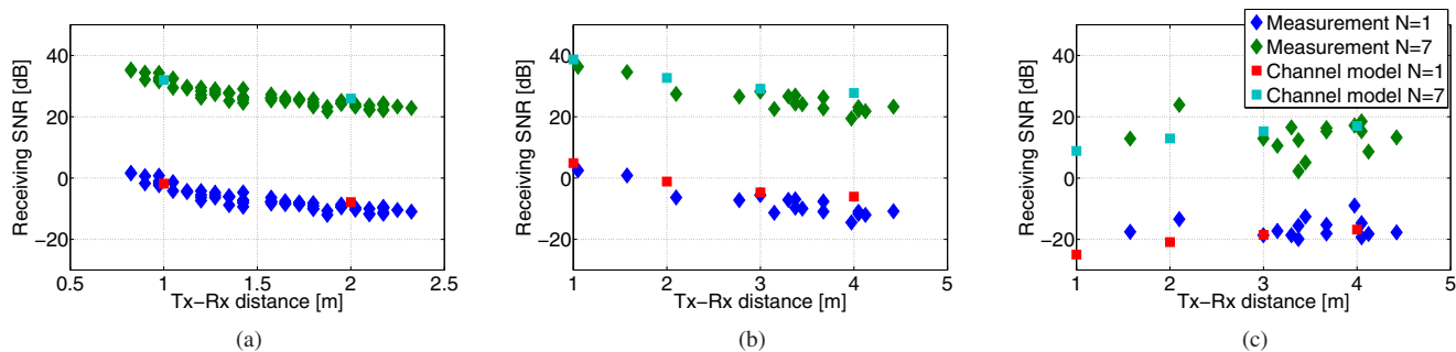
Fig. 2. Receiving SNR derived from channel measurements and the channel model for (a) LOS office, (b) LOS meeting room, and (c) NLOS meeting room scenarios.
