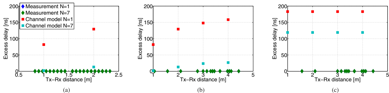
Fig. 3. Delay window derived from channel measurements and the channel model for (a) LOS office, (b) LOS meeting room, and (c) NLOS meeting room scenarios. Notice that the delay window was close to zero regardless of the use of beamforming in the measured channels, hence the two types of lozenges are totally overlapping in the figure.
