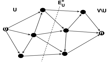
Fig. 1. An origin/destination cut of the network: \mathcal{U} is a subset of nodes including the origin 0 but not the destination n , and \mathcal{E}_\mathcal{U}^+ is the subset of those edges with tail node in \mathcal{U} , and head node in \mathcal{V} \setminus \mathcal{U} .
