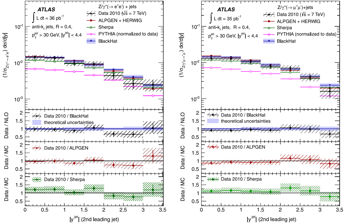
FIG. 10 (color online). Measured normalized jet cross section (1/\sigma_{Z/\gamma^* \rightarrow e^+e^-})d\sigma/d|y| (black dots) in (left) Z/\gamma^* \rightarrow e^+e^- + jets and (right) Z/\gamma^* \rightarrow \mu^+\mu^- + jets production as a function of the second-leading jet |y| , in events with at least two jets with p_T > 30 GeV and |y| < 4.4 in the final state, and normalized by \sigma_{Z/\gamma^* \rightarrow e^+e^-} and \sigma_{Z/\gamma^* \rightarrow \mu^+\mu^-} Drell-Yan cross sections, respectively.
