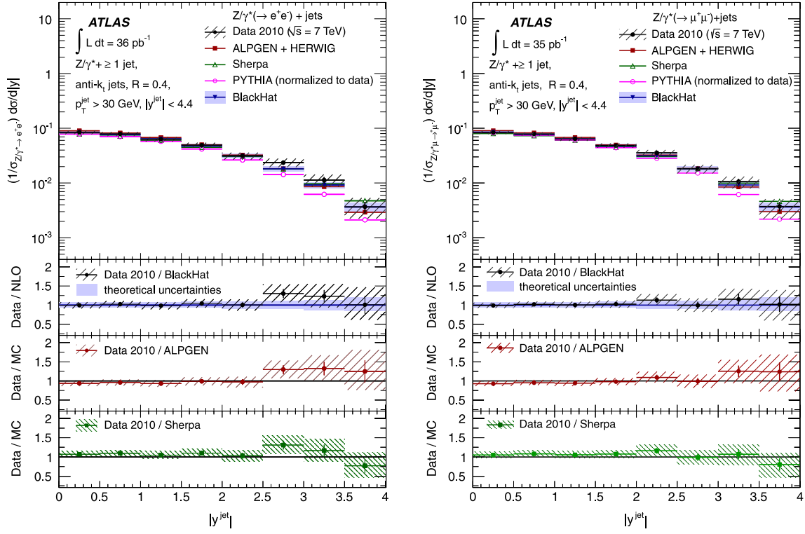
FIG. 8 (color online). Measured normalized inclusive jet cross section (1/\sigma_{Z/\gamma^* \rightarrow \ell^+ \ell^-}) d\sigma/d|y| (black dots) in (left) Z/\gamma^* (\rightarrow e^+ e^-) + \text{jets} and (right) Z/\gamma^* (\rightarrow \mu^+ \mu^-) + \text{jets} production as a function of |y| , in events with at least one jet with p_T > 30 GeV and |y| < 4.4 in the final state, and normalized by \sigma_{Z/\gamma^* \rightarrow e^+ e^-} and \sigma_{Z/\gamma^* \rightarrow \mu^+ \mu^-} Drell-Yan cross sections, respectively.
