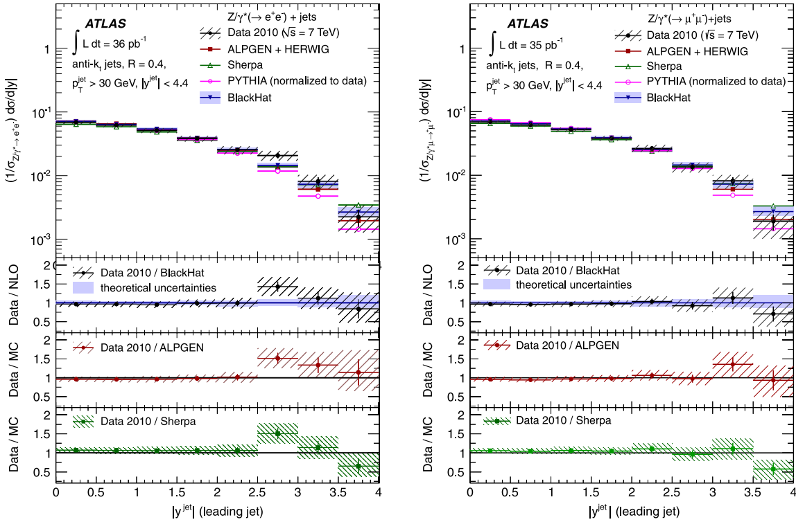
FIG. 9 (color online). Measured normalized jet cross section (1/\sigma_{Z/\gamma^* \rightarrow \ell^+ \ell^-}) d\sigma/d|y| (black dots) in (left) Z/\gamma^* (\rightarrow e^+ e^-) + \text{jets} and (right) Z/\gamma^* (\rightarrow \mu^+ \mu^-) + \text{jets} production as a function of the leading jet |y| , in events with at least one jet with p_T > 30 GeV and |y| < 4.4 in the final state, and normalized by \sigma_{Z/\gamma^* \rightarrow e^+ e^-} and \sigma_{Z/\gamma^* \rightarrow \mu^+ \mu^-} Drell-Yan cross sections, respectively.
