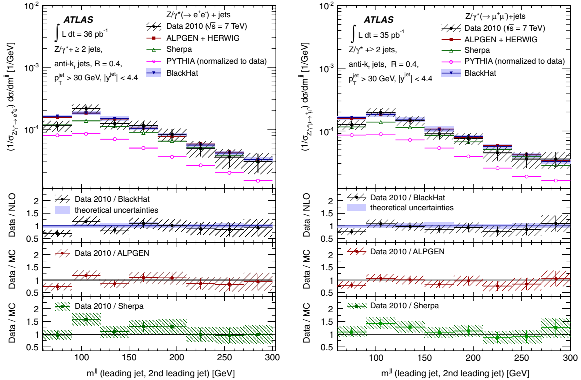
FIG. 11 (color online). Measured normalized dijet cross section (1/\sigma_{Z/\gamma^* \rightarrow e^+e^-})d\sigma/dm^{jj} (black dots) in (left) Z/\gamma^* \rightarrow e^+e^- + jets and (right) Z/\gamma^* \rightarrow \mu^+\mu^- + jets production as a function of the invariant mass of the two leading jets m^{jj} , in events with at least two jets with p_T > 30 GeV and |y| < 4.4 in the final state, and normalized by \sigma_{Z/\gamma^* \rightarrow e^+e^-} and \sigma_{Z/\gamma^* \rightarrow \mu^+\mu^-} Drell-Yan cross sections, respectively.
