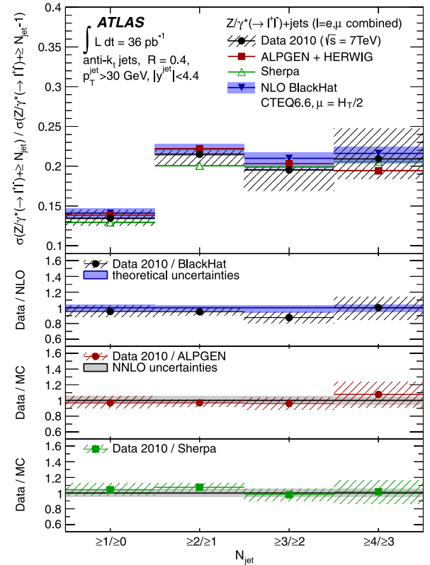
FIG. 16 (color online). Measured ratio of cross sections (\sigma_{N_{\text{jet}}}/\sigma_{N_{\text{jet}}-1}) (black dots) in Z/\gamma^* \rightarrow \ell^+ \ell^- + \text{jets} production as a function of the inclusive jet multiplicity, for events with at least one jet with p_T > 30 GeV and |y| < 4.4 in the final state.
