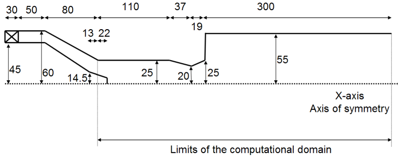
Figure 4.1: Schematics of the Lisbon burner. Lengths in [mm] [23,24].
