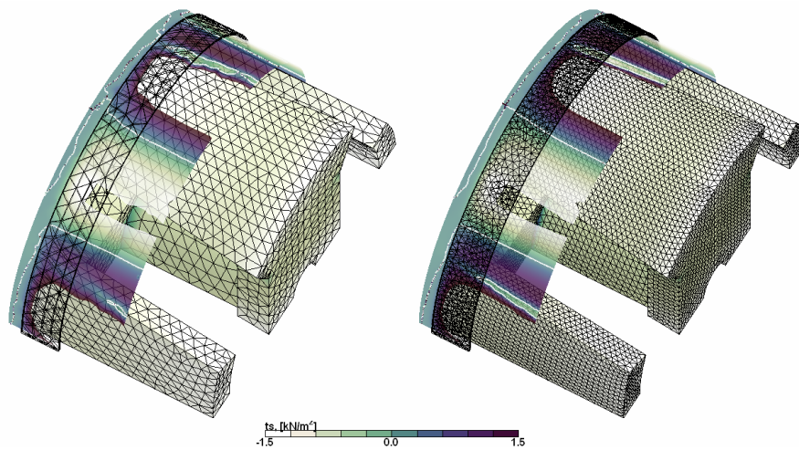
Figure C.9: Shear force distribution dependence on the tetrahedral elements. White lines indicate the region where the force changes sign.
