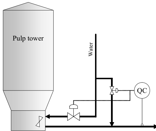
Figure 6.8 The consistency in the pulp tower is typically 8–12 %. Dilution to pumpable suspension takes place at the bottom of the tower by injection of dilution water. An agitator helps the mixing.
