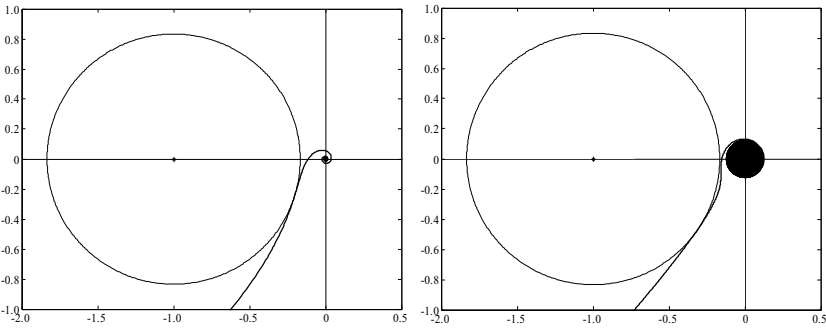
Figure 5.18 Nyquist curves for the marked controllers in Table 5.2 and the process in (5.16), PI – left, PID – right. An often occurring difference between the two optimized Nyquist curves is that for the PID controller the curve touches the M_s -circle in two points but only once for the PI controller. This can also be seen in the sensitivity function in Figure 5.17.
