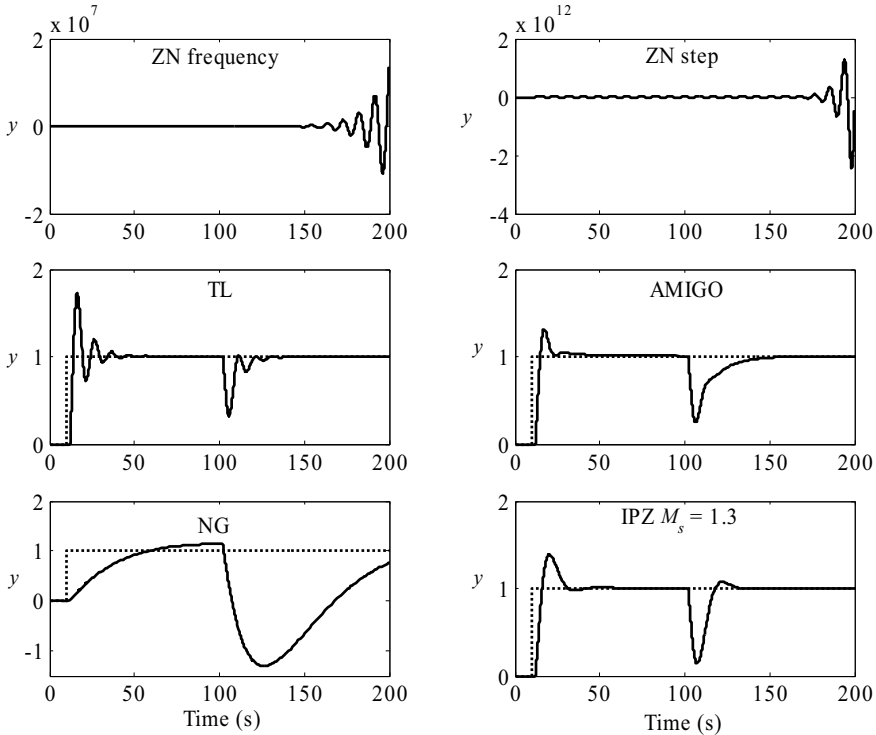
Figure 5.32 Robustness analysis of the tuning methods used in comparison with the IPZ tuning. The time delay in (5.17) is changed from 1 to 2 seconds.
