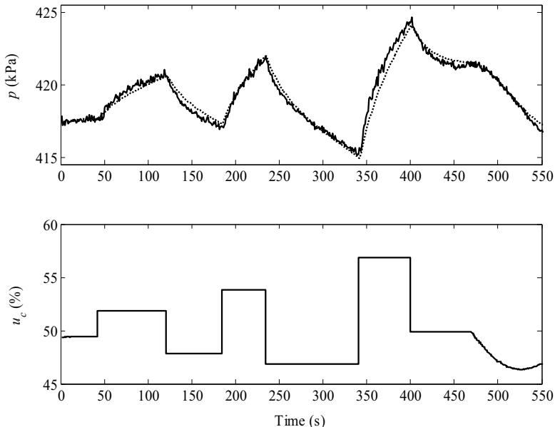
Figure 4.4 Calibrated model (dotted) and measured data (solid).
