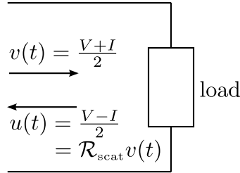
Figure 6: In this case, the input v(t) and output u(t) are the amplitudes (measured by the load) of the voltage waves traveling towards and from the load, respectively. They are related by the scattering (or reflection) operator \mathcal{R}_{\text{scat}} . The absorbed energy is given by (2.10).
