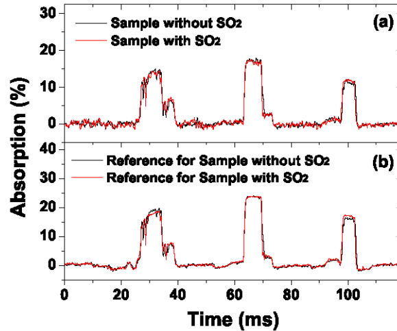
Fig. 8. (a) Sample absorption signals of mercury vapor with and without interference by \text{SO}_2 (2000 ppm, 10 cm) and (b) corresponding reference signals.
