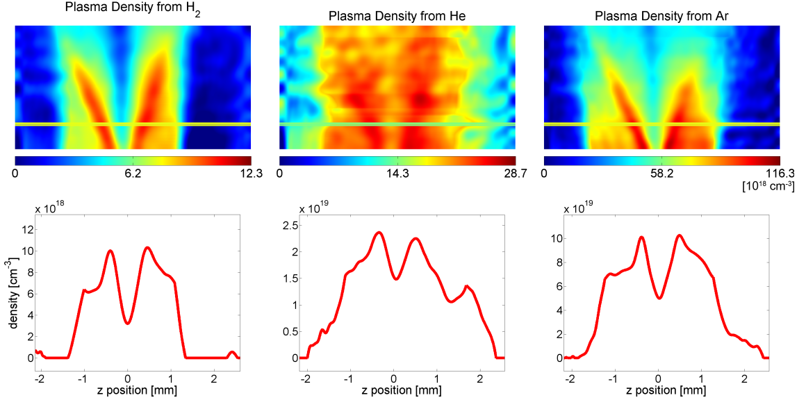
Figure 4.2. Qualitative comparison of plasma densities obtainable with H_2 , He and Ar flowing around a 50\mu m diameter wire. The gas is released through a 3 mm supersonic nozzle with 10 bar backing pressure: Top: Density maps with diverging compression waves, caused by the wire. The plasma densities are for a fully ionised gas. Bottom: Lineout of plasma densities at laser interaction height. One can distinguish different fluid characteristics of the gases around the obstacle, leading to a variation in the relative depth of the density depletion centrally above the obstacle.
