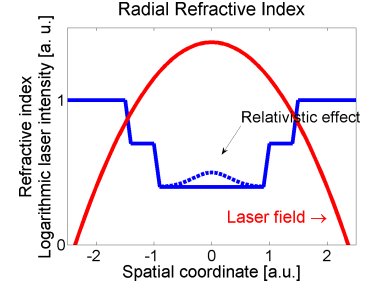
Figure 2.3. Schematic of \eta(r) (blue) decreasing in steps whenever laser intensity (red, logarithmic) exceeds a threshold level and a new atomic shell can be ionized. In a highly relativistic plasma response, the electrons however create a guiding channel on the axis.
