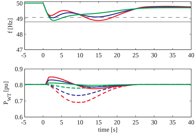
Figure 7.8 30 000 MW load, 12 000 MW wind power production, loss of 1 400 MW thermal production. \Delta f -controller with t_{inc}=2 s and t_{dec}=20 s. P_{inc}=0.01 (green), P_{inc}=0.03 (blue), P_{inc}=0.05 (red). Black dashed line indicates lowest frequency without wind power and black solid line with uncontrolled wind power. At the bottom dashed lines are P_{order} and solid lines are P_{ref} .
