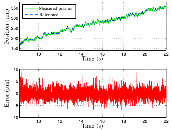
Fig. 6. Reference and position of the micro manipulator during milling experiment in the y -direction (upper panel) and corresponding control error (lower panel).
