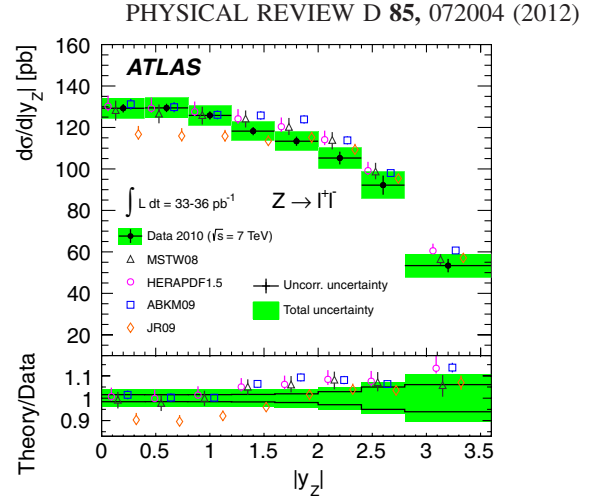
FIG. 12 (color online). Differential d\sigma/d|y_Z| cross section measurement for Z \rightarrow \ell\ell compared to NNLO theory predictions using various PDF sets. The kinematic requirements are 66 < m_{\ell\ell} < 116 GeV and p_{T,\ell} > 20 GeV. The ratio of theoretical predictions to data is also shown. Theoretical points are displaced for clarity within each bin.
