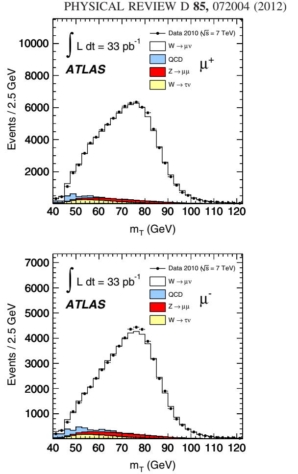
FIG. 8 (color online). Transverse mass distribution of candidate W^+ (top panel) and W^- (bottom panel) events. The simulation is normalized to the data. The QCD background shape is taken from simulation and normalized to the number of QCD events measured from data.
