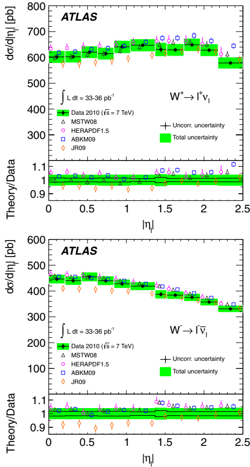
FIG. 13 (color online). Differential d\sigma/d|\eta_{\ell^+}| (top panel) and d\sigma/d|\eta_{\ell^-}| (bottom panel) cross section measurements for W \rightarrow \ell \nu compared to the NNLO theory predictions using various PDF sets. The kinematic requirements are p_{T,\ell} > 20 GeV, p_{T,\nu} > 25 GeV, and m_T > 40 GeV. The ratio of theoretical predictions to data is also shown. Theoretical points are displaced for clarity within each bin.
