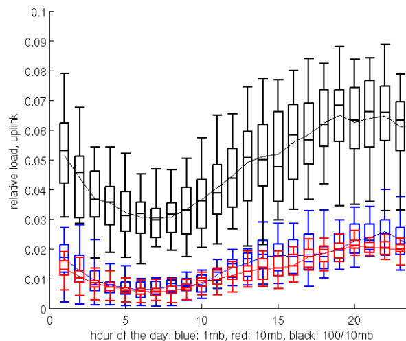
Figure 2. Average daily load per ST in the uplink direction for the 1 Mbps, 10 Mbps and 100/10 Mbps STs.
